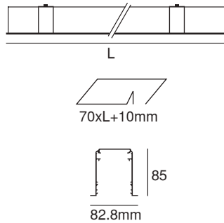
82.8mm RECESSED LINEAR
