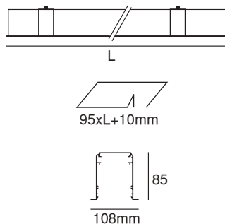
108mm RECESSED LINEAR
